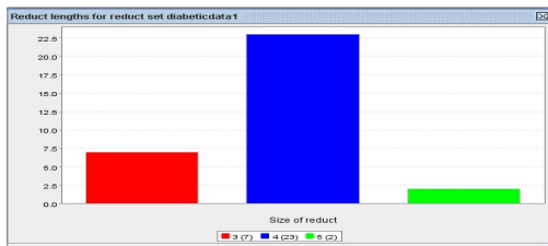
Figure 4. Reduct Length for the reduct set
